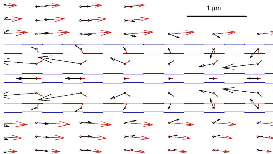
Figure 1: 2D FDTD simulation of Poynting vector of the “photonic syringe”. Light injection is from the left side. Excitation is narrowband (vacuum wavelength \lambda_0 \approx 1.5 \mu\text{m} ). Map is to scale. Only a few periods are shown, in proximity of the input side. Red (black) arrows show the result without (with) corrugation. The blue lines are the outline of the structure with corrugation. While the energy in the outer side of the waveguide is always traveling forward (top and bottom of figure), in the slots (i.e., in the 2 regions between the slabs), the component along the waveguide axis is dominantly forward (backward) in absence (presence) of the corrugation.
